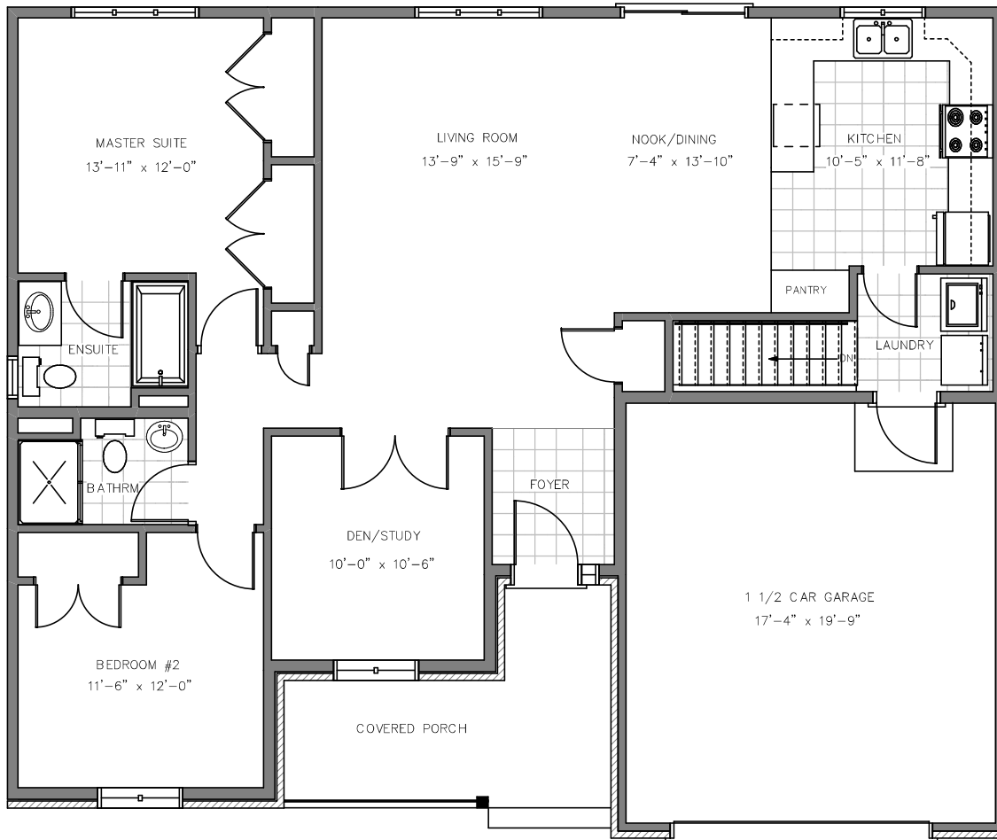
THE NEWBEDFORD MAIN FLOOR PLAN 1304 SQ. FT.
