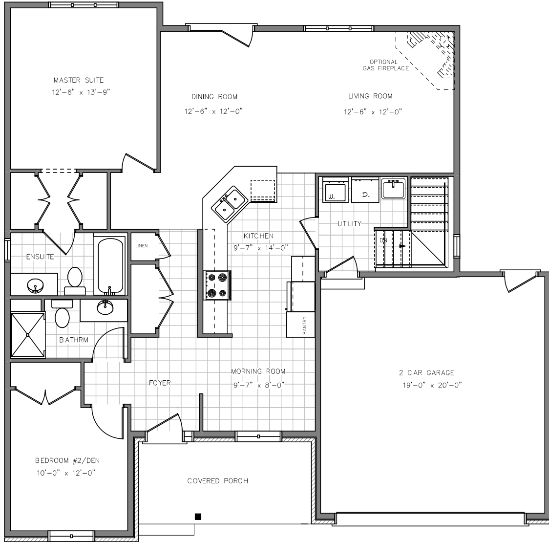
THE GEORGETOWN MAIN FLOOR PLAN 1336 SQ. FT.
